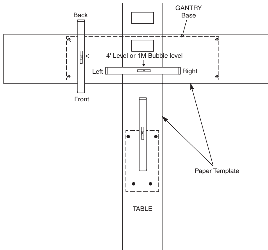
Figure 1-3 Check Floor Level
