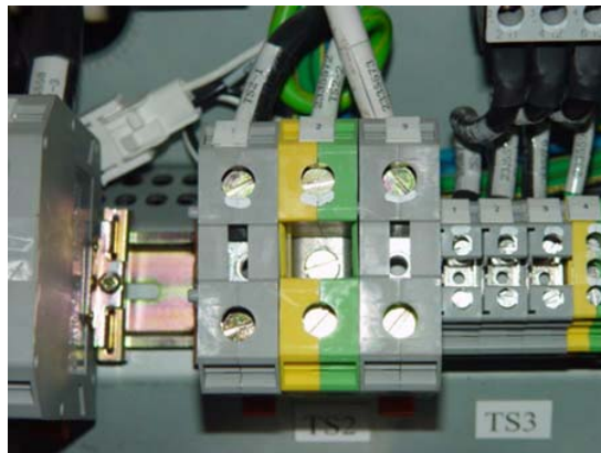
Figure 2-24 HVDC Connection
