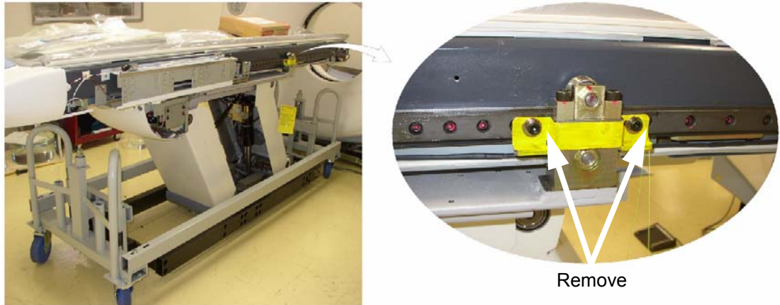
Figure 1-45 IMS Shipping Lock
