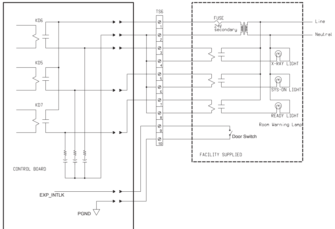
Figure 2-28 Typical TS6 Warning Light &amp; Door Interlock Connections
