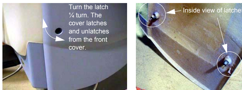
Figure A-1 Side Cover Latches
