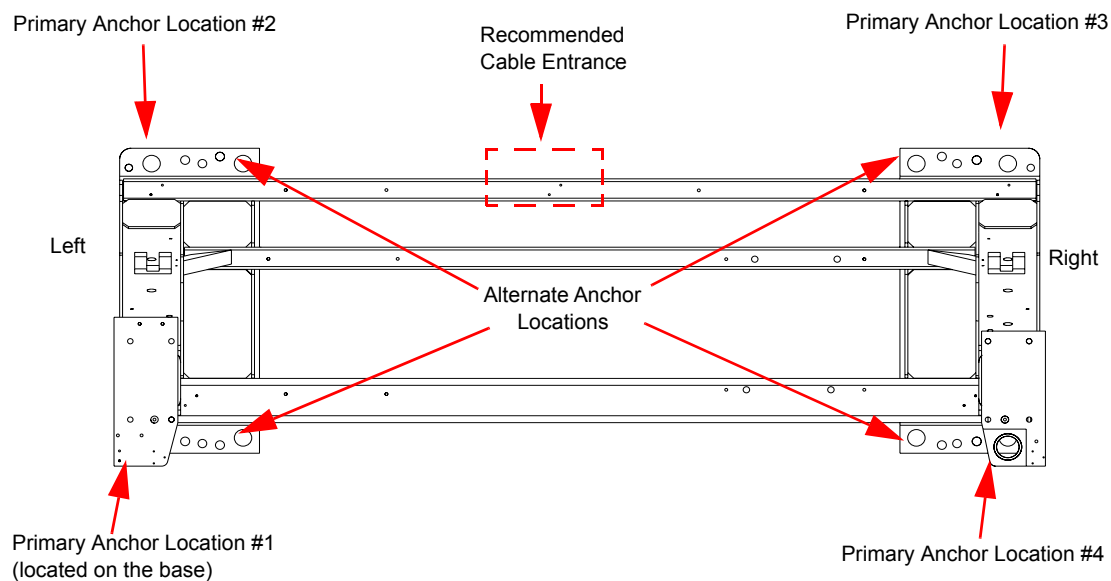
Figure 1-40 Anchor Locations
