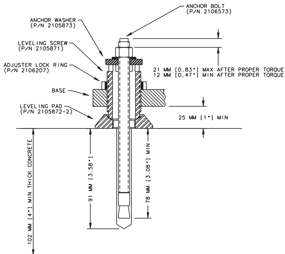
Figure 1-41 Typical Floor Anchor, Gantry and Table (GT 1700/GT2000)
