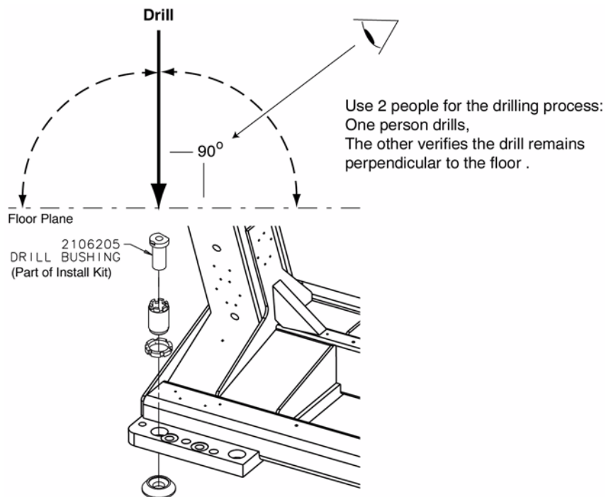
Figure 1-39 Drilling Position
