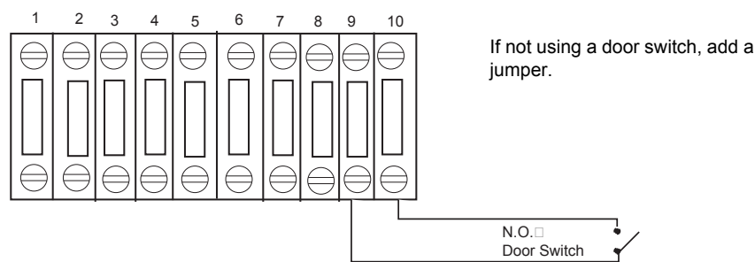
Figure 2-30 With a Door Interlock
