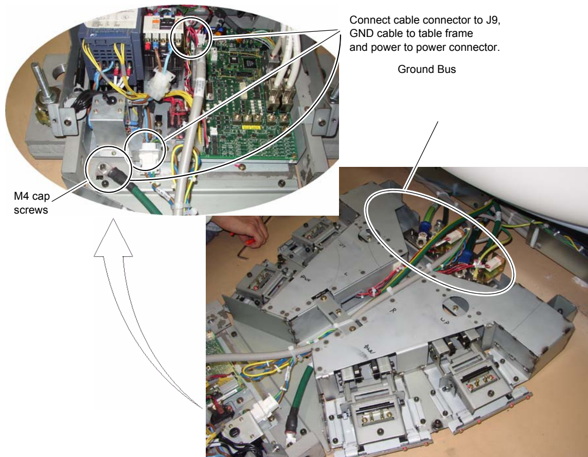
Figure 1-54 Footswitch Assembly Cable Wiring
