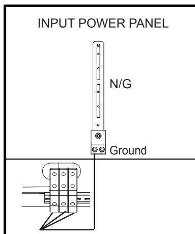
Figure 2-21 Input Power Panel Connections
