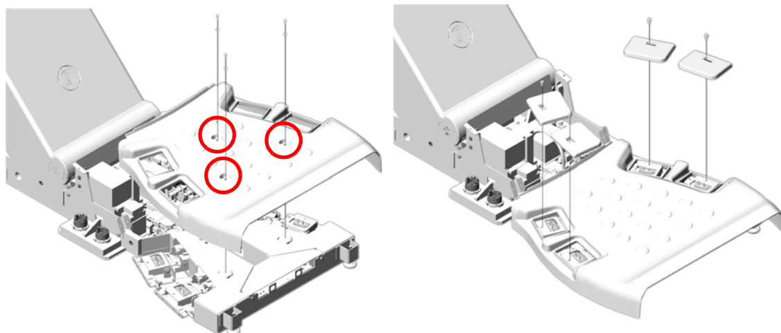
Figure 1-56 Footswitch Cover Installation
