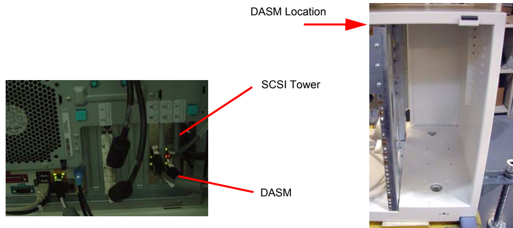
Figure 2-11 Rear view of HP xw8200, showing DASM SCSI cable connection
