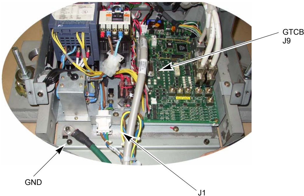
Figure 2-18 Table Connections
