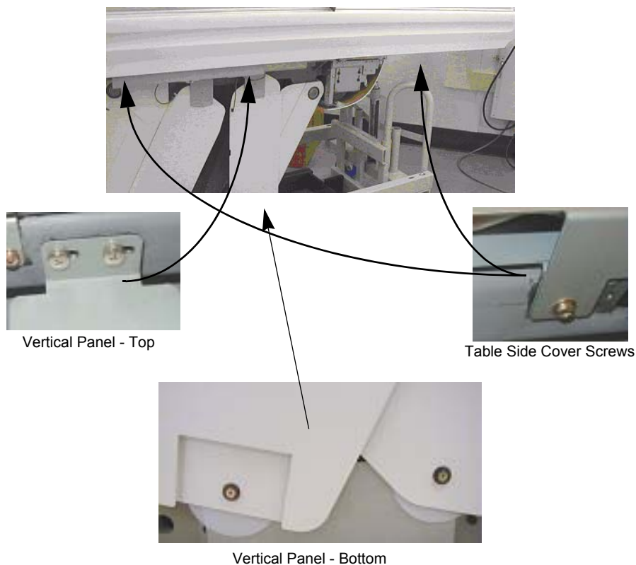
Figure 1-27 Table Covers
