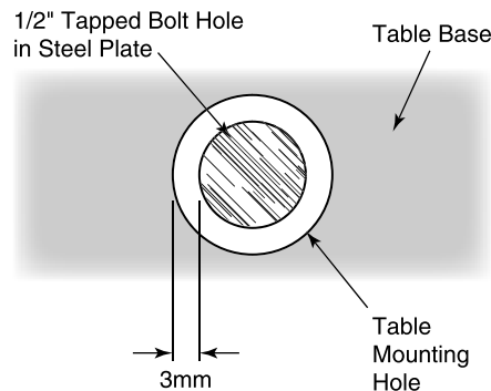
Figure 1-44 Center tapped holes under mounting holes in table base
