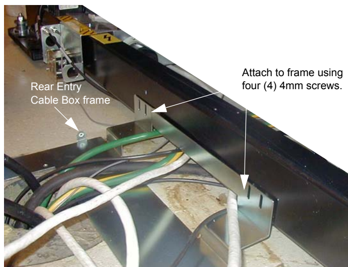
Figure 1-50 Rear Entry Cable Box
