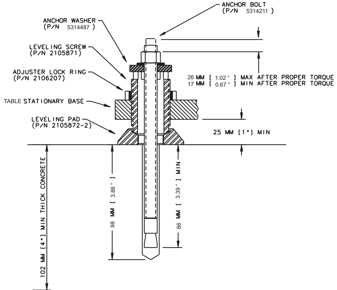
Figure 1-42 Typical Floor Anchor, Table (GT650lbs)
