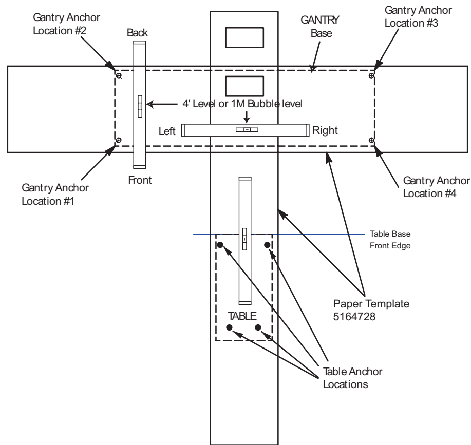
Figure 1-5 Anchor Hole Locations
