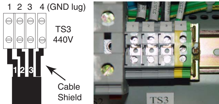
Figure 2-25 440VAC Connection
