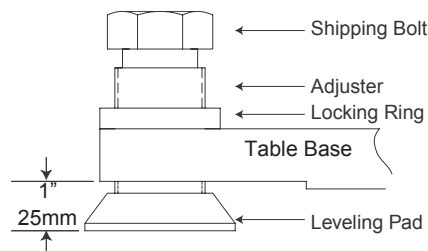
Figure 1-25 Table Base Leveling Pads (Starting Positions)
