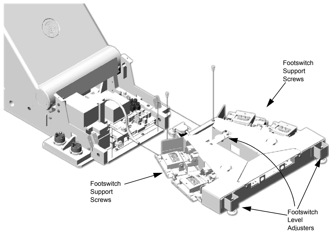
Figure 1-51 Footswitch Assembly Installation
