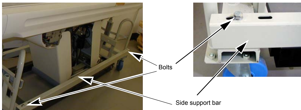
Figure 1-46 Dolly Bolts
