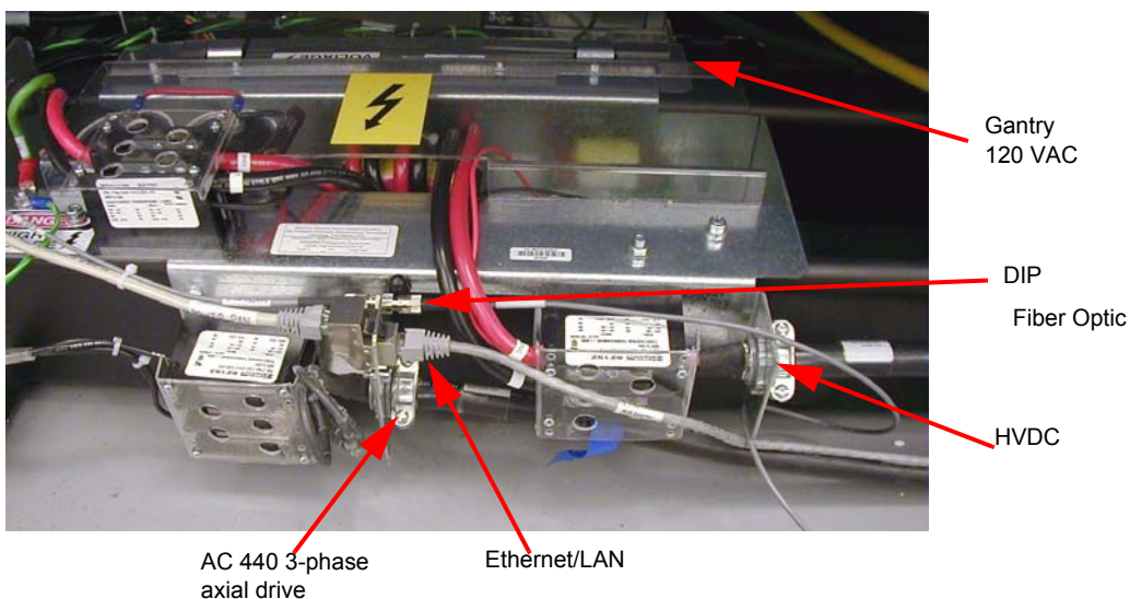
Figure 2-15 Gantry Power Pan
