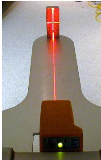
Figure 1-22 Laser Centering
