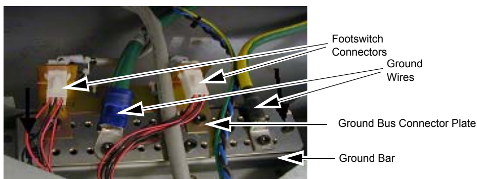
Figure 1-55 Footswitch Ground/Bus Bar
