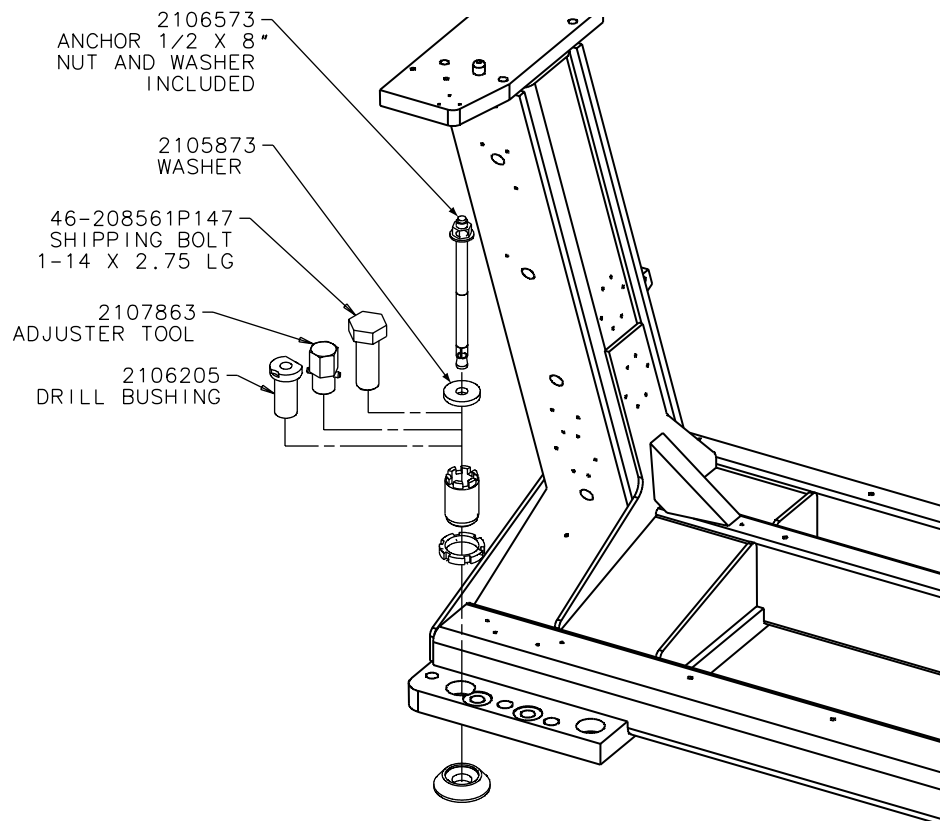
Figure 1-6 Gantry Base Installation Hardware
