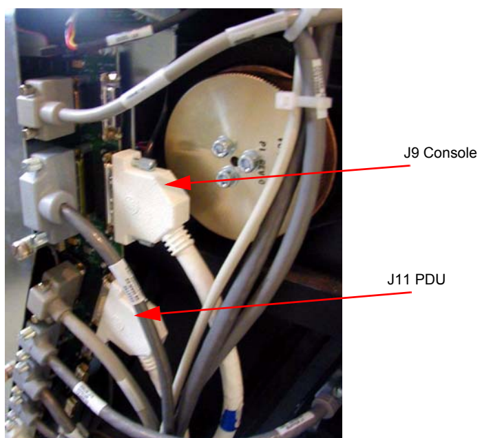
Figure 2-17 TGPU Connections
