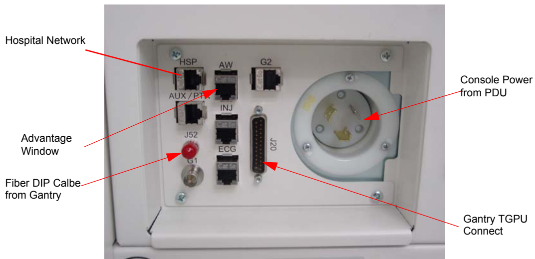
Figure 2-9 Power Connections
