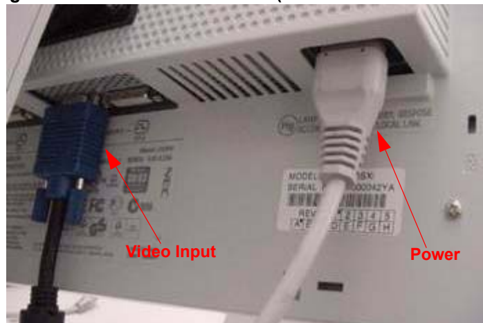
Figure 2-8 Monitor Connections (NEC Model LCD 1980SXi)
