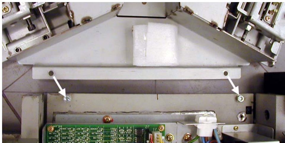
Figure 1-52 Attach Footswitch
