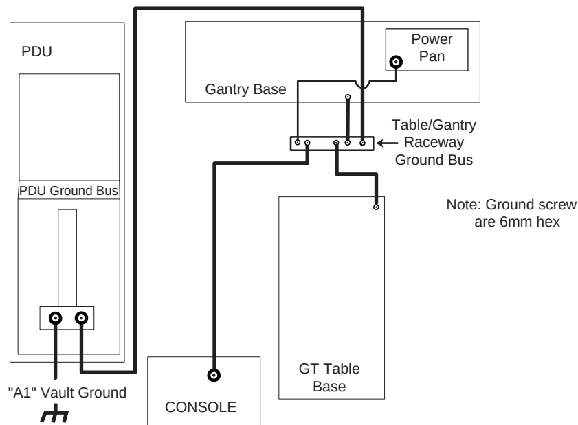
Figure 2-31 CT System Ground Connections
